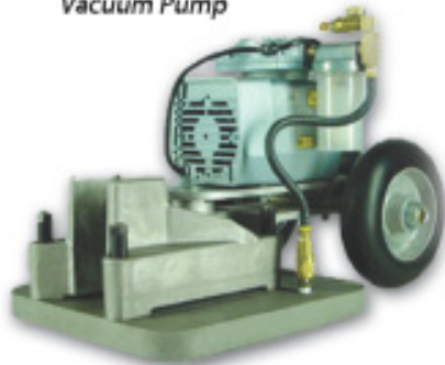
Core Drill Base Assembly with Vacuum Pump
